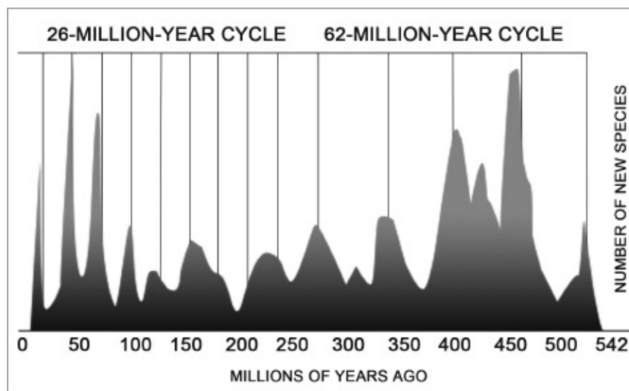
Fig. 2: Combined graph of 26- and 62-million-year evolution cycles
