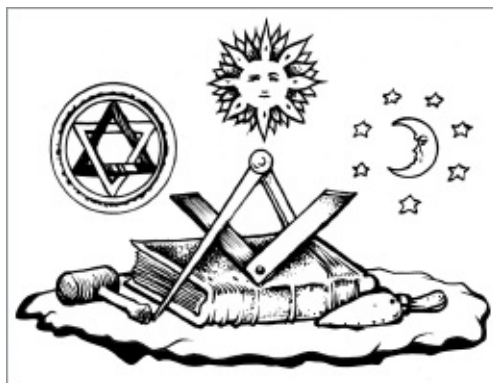
Fig. 25 : This is another one of many Masonic illustrations showing the Sun, the Moon, and a companion star.
